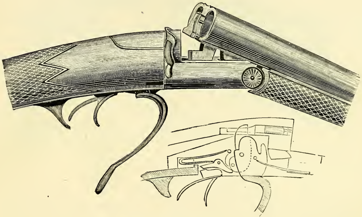
Green's Hammerless Gun.
